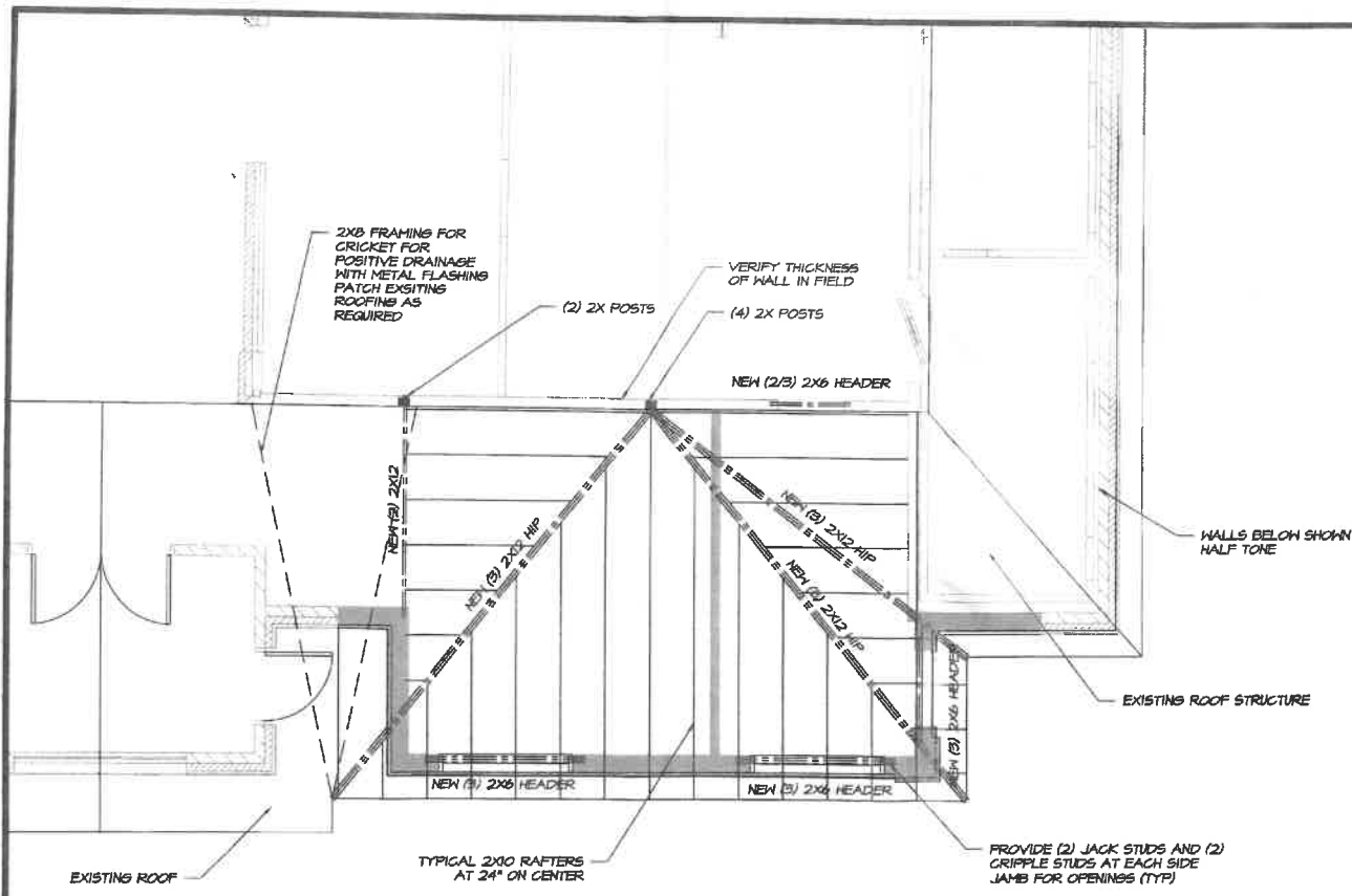
Roof Framing Plan 1/4" = 1'-0"
