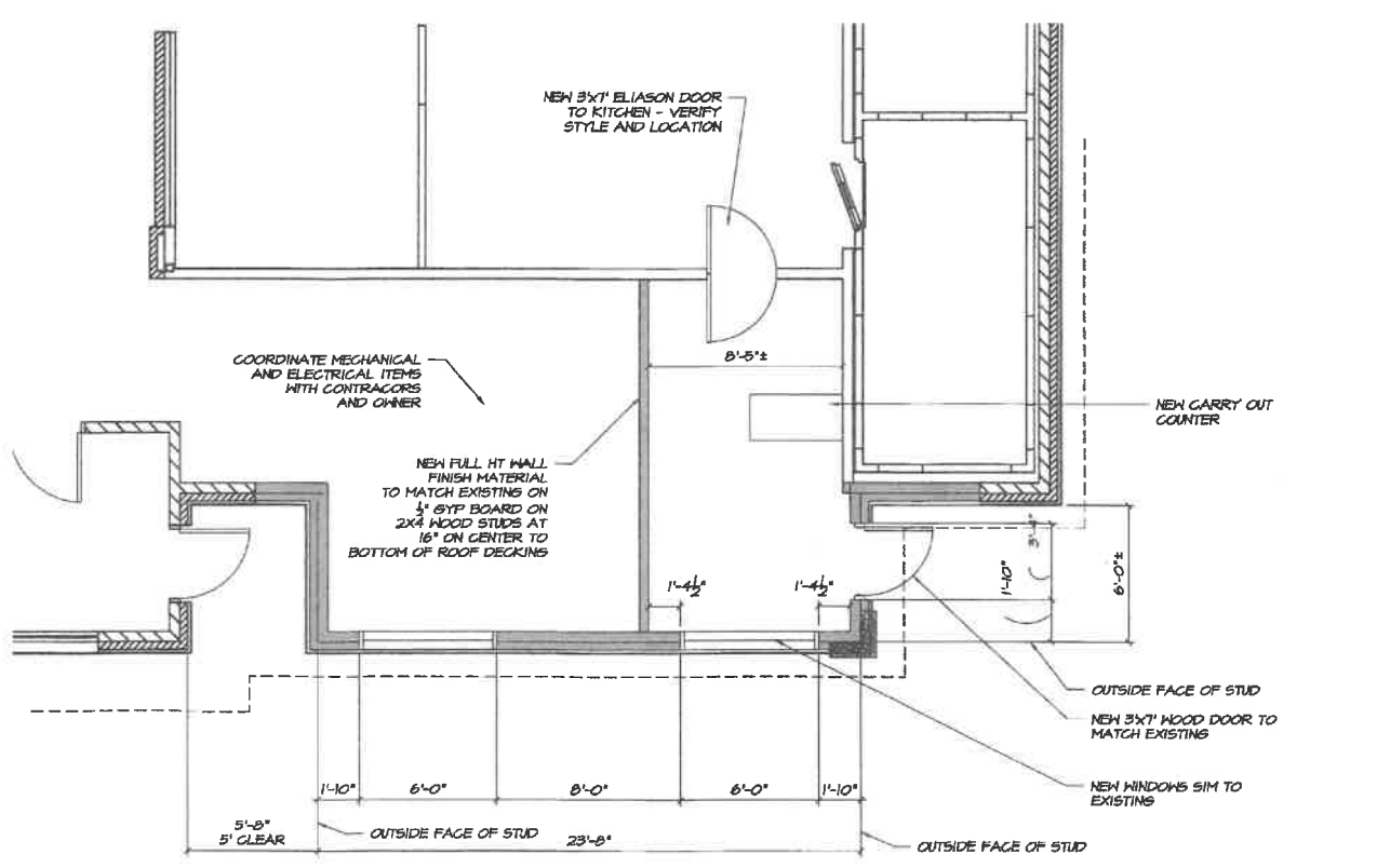
Proposed Floor Plan 1/4" = 1'-0"
