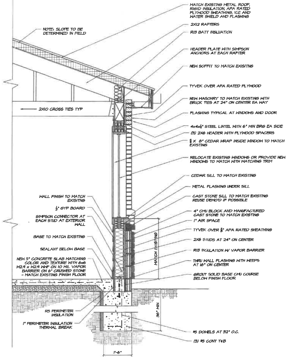
1 Typical Wall Section 3/4"=1'-0"
