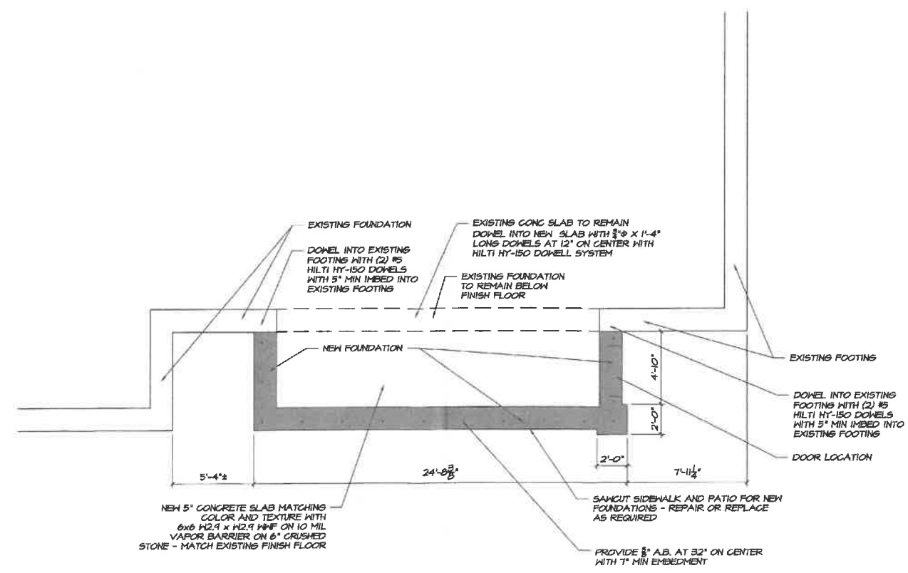
Foundation Plan 1/4" = 1'-0"
